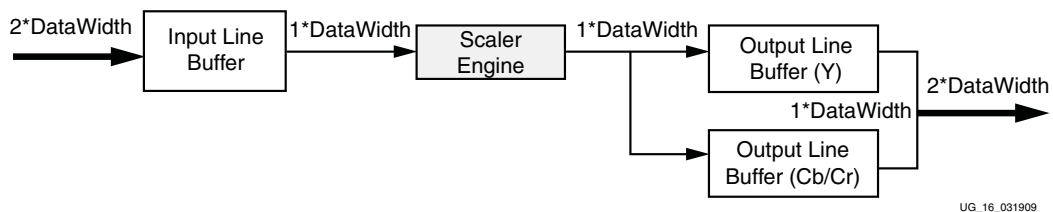
Figure 3-4: Internal Data Path Bitwidths for Single-Engine YC Mode
