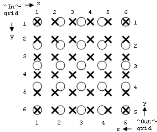
Figure 3-2: 5x5 Output Grid (“O”) Super-imposed over 6x6 Input Grid (“X”)
