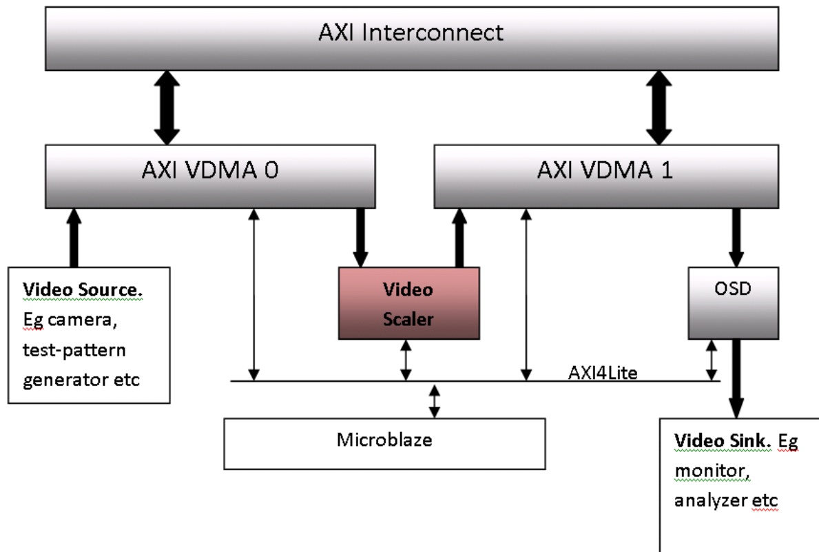
Figure 10-1: Simplified System Diagram
