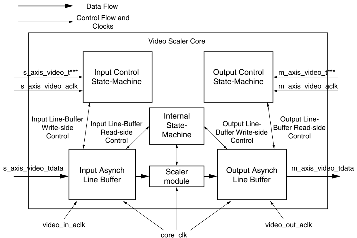
Figure 3-7: Block Diagram Showing Clock Domains
