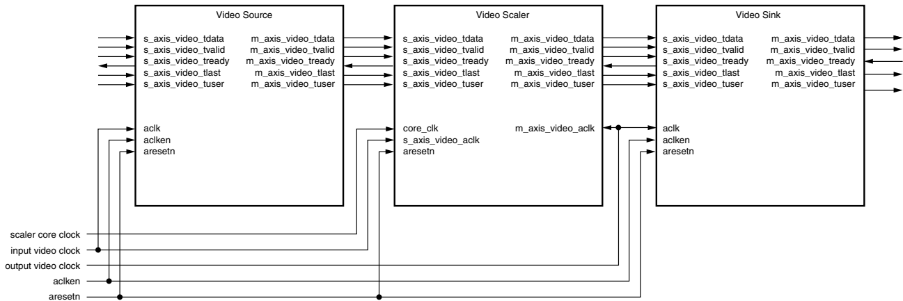
Figure 3-8: Video Scaler Example
