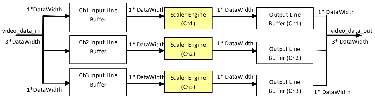
Figure 3-6: Internal Data Path Bitwidths for Triple-Engine RGB/4:4:4 Architecture
