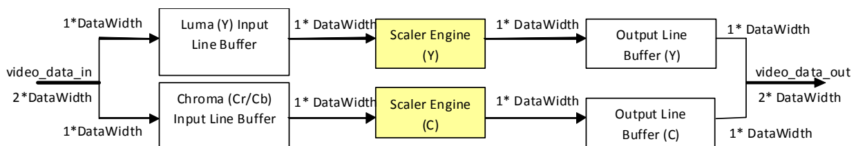
Figure 3-5: Internal Data Path Bitwidths for Dual-Engine YC Mode
