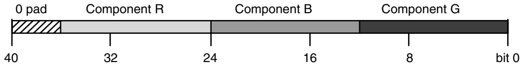
Figure 2-3: RGB Data Embedding on TDATA
