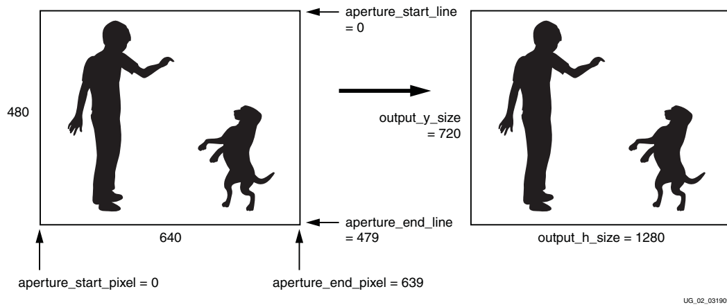
Figure 10-3: Format Up-scaling. Example 640x480 to 720p, HSF = 2^{20} \times 640/1280 ; 2^{20} \times VSF = 480/720
