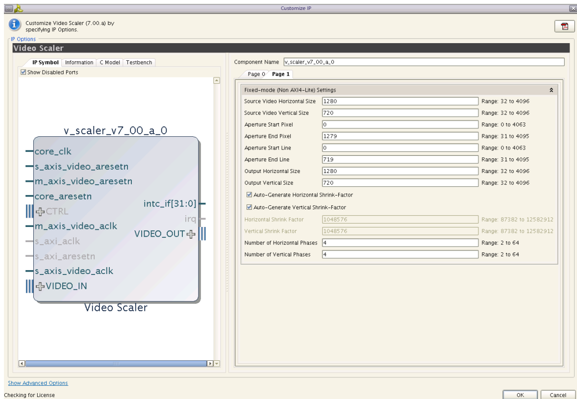
Figure 5-2: Video Scaler Graphical User Interface for Constant Mode (page 2)
