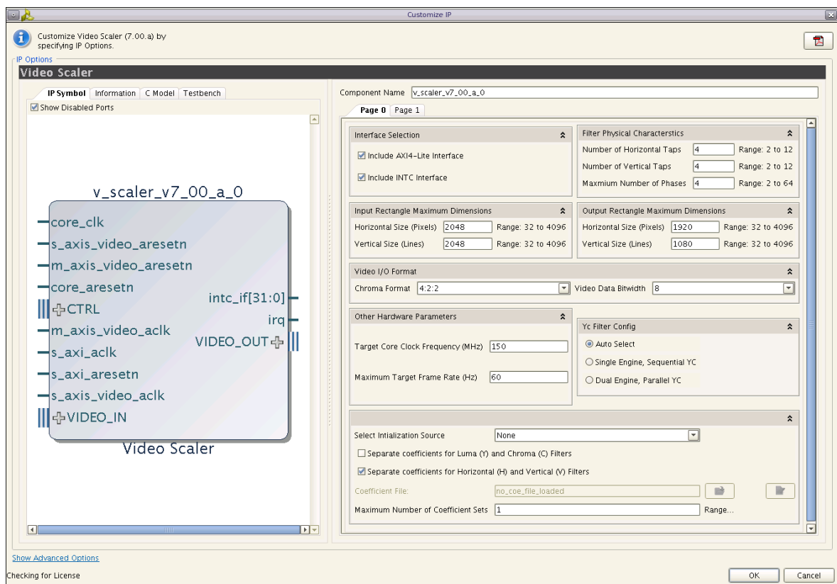
Figure 5-1: Video Scaler Main Screen
