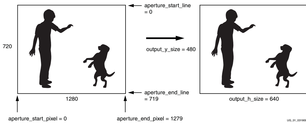
Figure 10-2: Format Down-scaling. Example 720p to 640x480, HSF = 2^{20} \times 1280/640 ; VSF = 2^{20} \times 720/480
