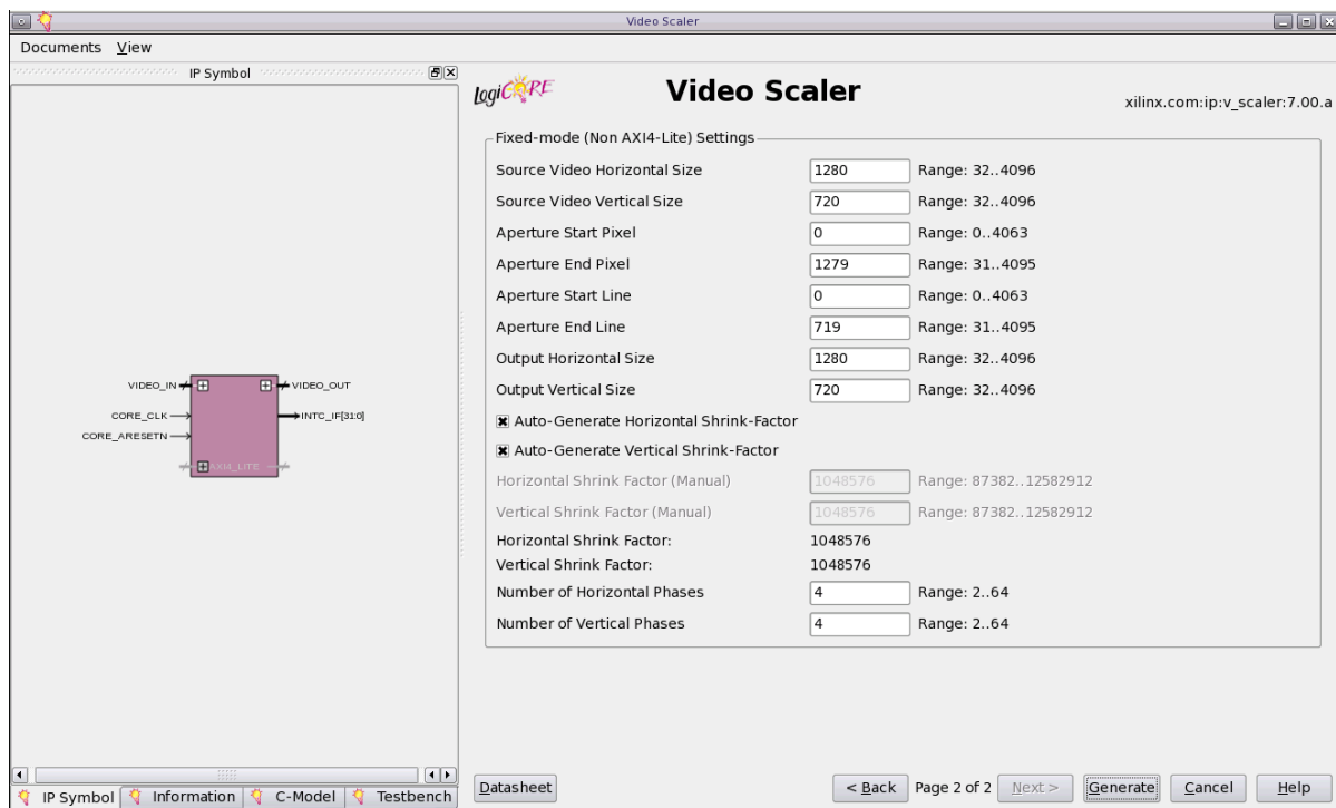
Figure 8-2: Video Scaler Graphical User Interface for Constant Mode (page 2)
