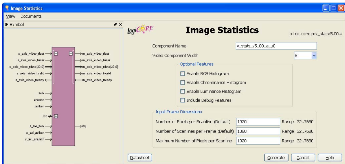
Figure 7-1: Image Statistics CORE Generator GUI
