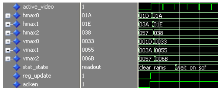
Figure D-2: Register Update Example
