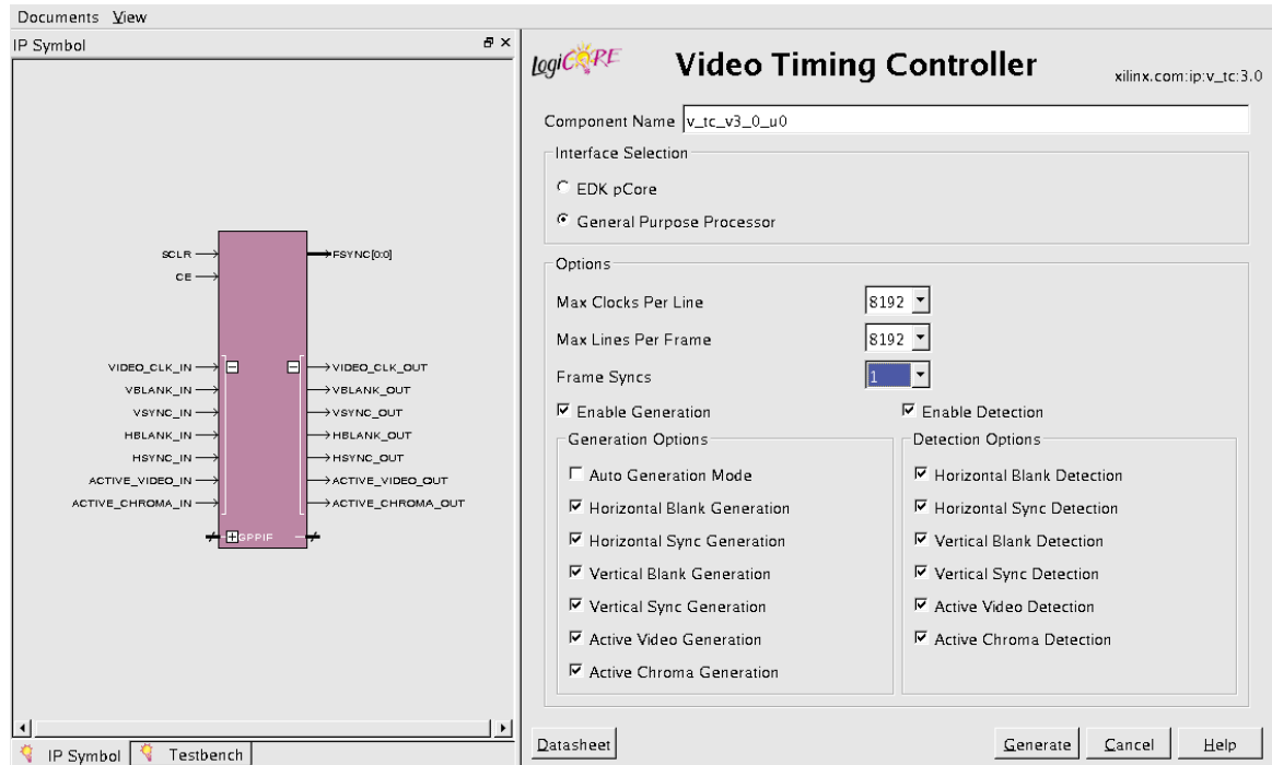
Figure 2: Video Timing Controller Graphical User Interface
