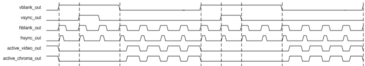
Figure 6: Generated Vertical Timing (4:4:4 Chroma)
