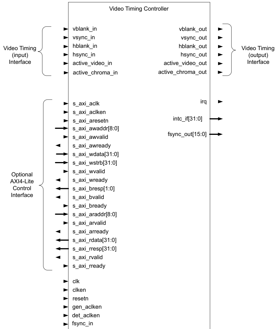
Figure 2-1: TC Core Top-Level Signaling Interface
