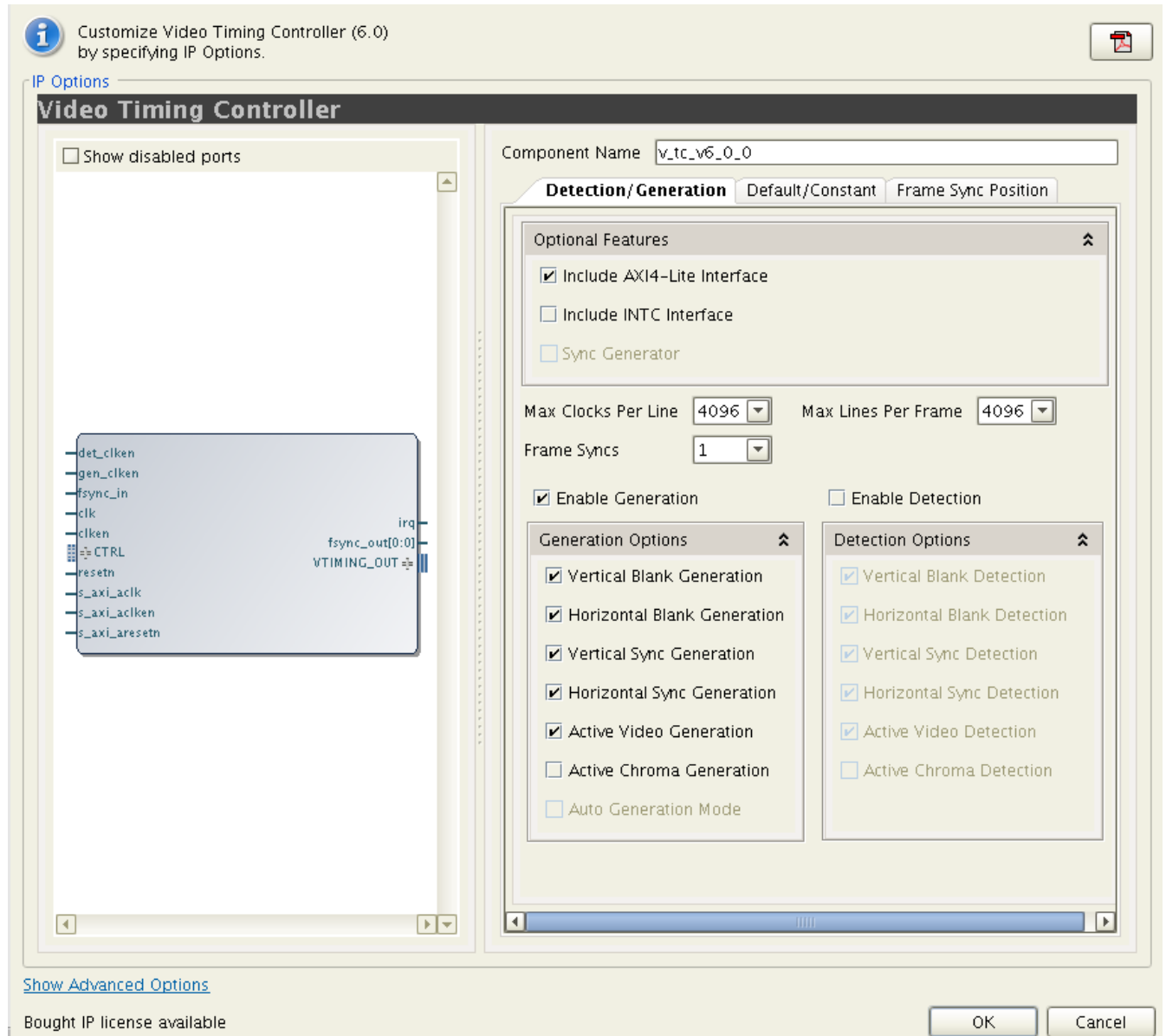
Figure 4-1: Vivado GUI Screen
