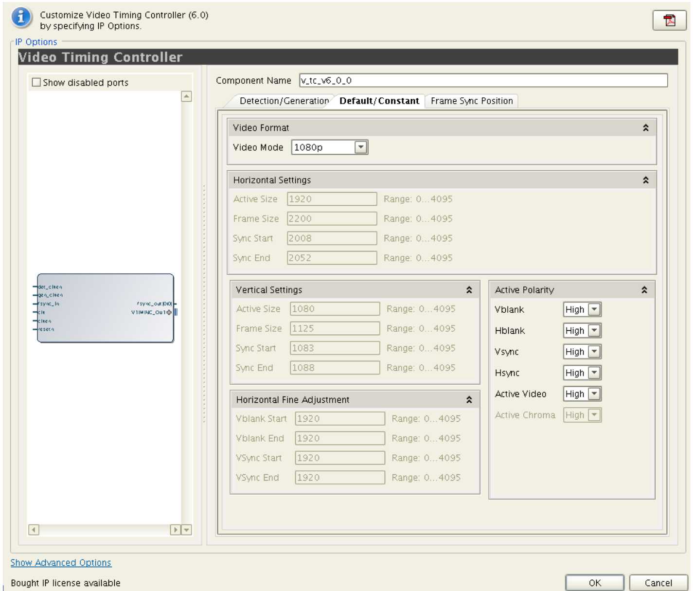
Figure 4-2: Second Vivado Screen
