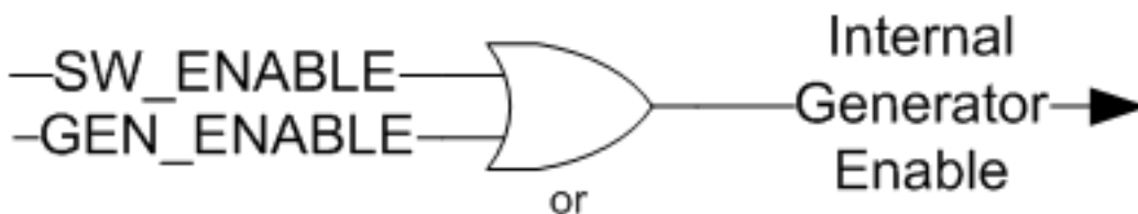
Figure 2-6: Generator Internal Enable Logic
