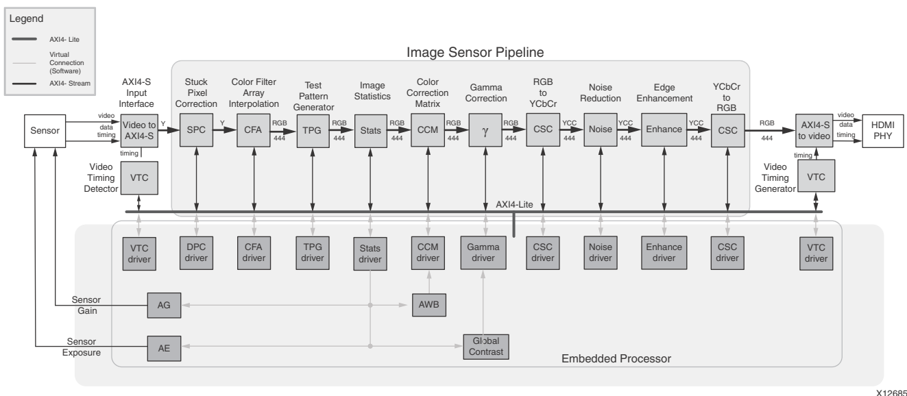
Figure 3-1: Image Sensor Pipeline System with YCrCb to RGB Core
