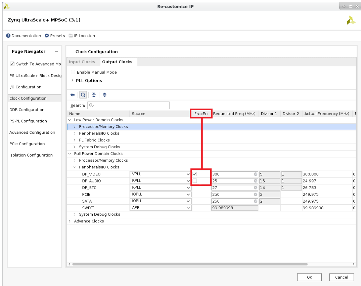
Figure 4-10: FracEnable
