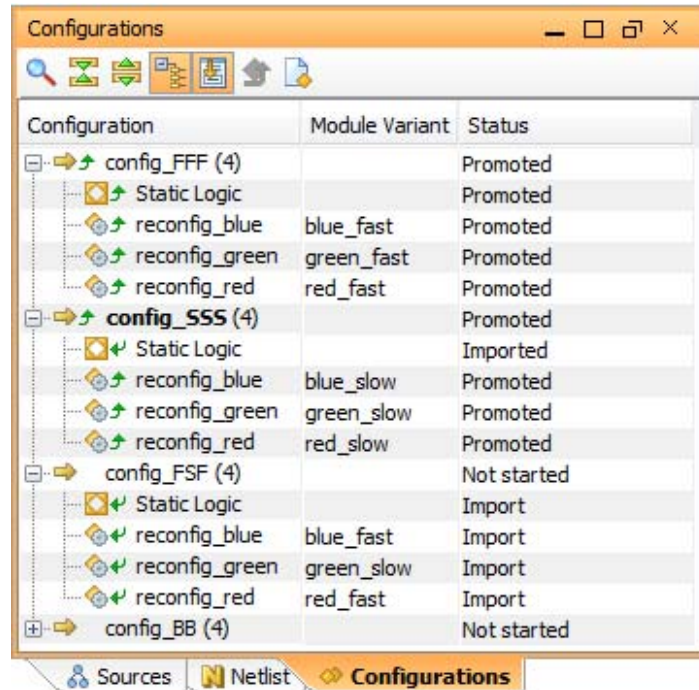
Figure 4-36: Multiple Configurations Promoted
