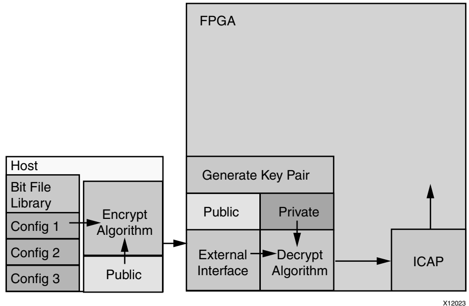
Figure 2-6: Loading an Encrypted Partial Bit File
