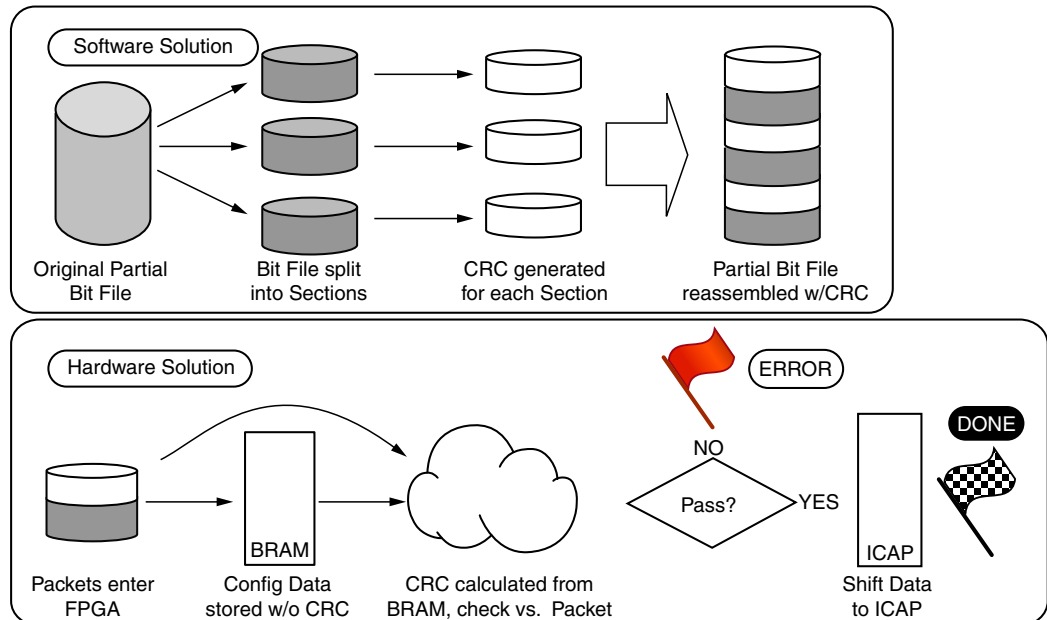
Figure 6-5: CRC Checking for a Partial Reconfiguration Design
