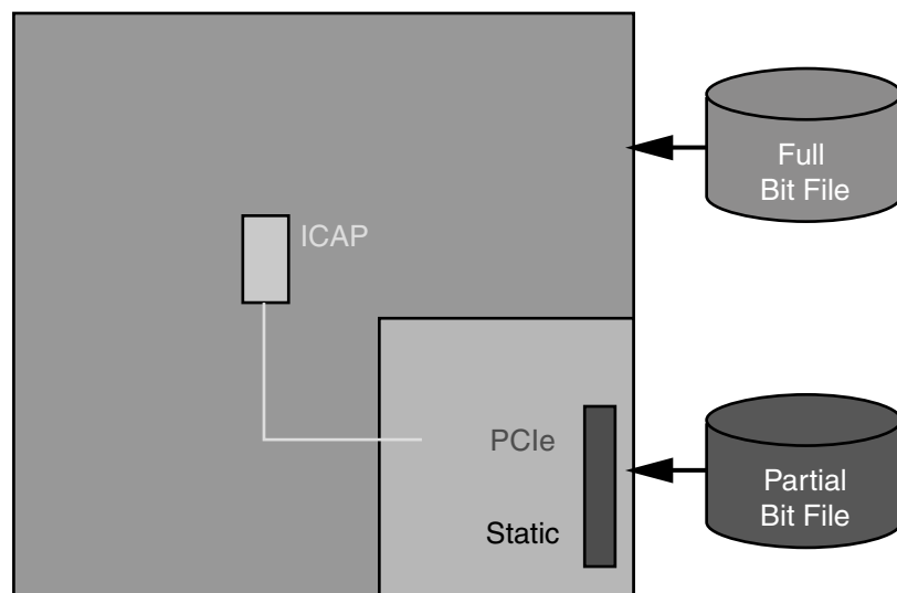
Figure 2-3: Configuration by Means of PCIe Interface
