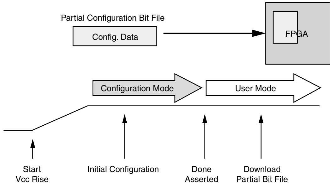
Figure 6-2: Configuring With a Partial Bit File
